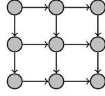
Fig. 9. Grid graph.
