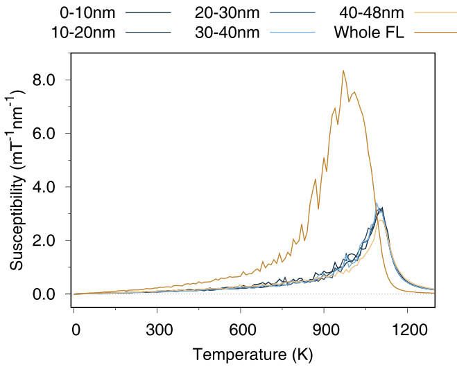
Figure 3. Susceptibility against temperature for the whole 48 nm FL (as in figure 2), compared to local 10 nm thick sections of the free layer. The localised curves are all the same order of magnitude and width (with the 8 nm section slightly reduced) when compared to the whole FL. This demonstrates that locally, the spins are correlated, so the noise in the whole FL is a consequence of variation in the spin direction or non-uniform excited modes.
