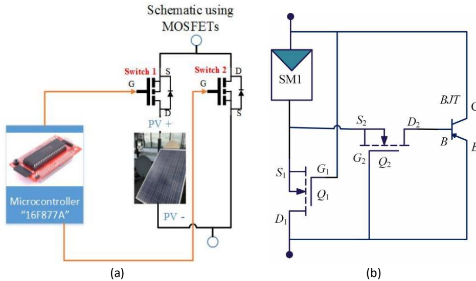
Fig. 2. PV hotspot mitigating techniques, (a) Dual MOSFET concept [16], (b) BJT-Based bypass concept [19].
