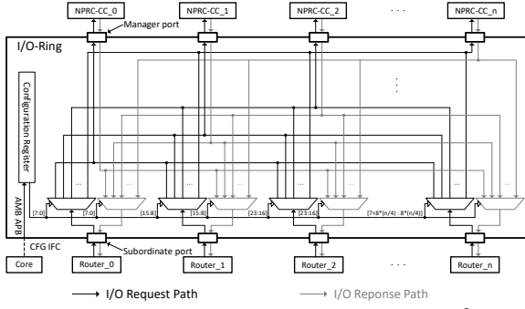
Figure 3: Micro-architecture of I/O-Ring in R 2 NoC.
