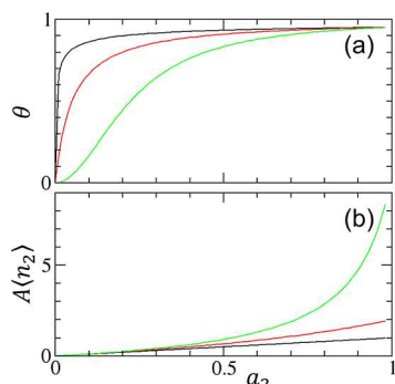
Figure 1. (a) Convergent cooperativity. The fractional coverage \theta of the cooperative isotherm (eq 7) is plotted against the activity of sorbate ( a_2 ) with the parameters A_m = 20 and m = 0.5 (black), 1.0 (red), and 2.0 (green). (b) Divergent cooperativity. The normalized amount of sorption ( A\langle n_2 \rangle ) of the AB isotherm (eq 14b) is plotted against a_2 with the parameters K_b = 0 (black), 0.5 (red), and 0.9 (green).
