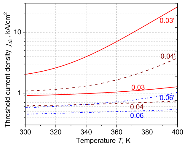
Fig. 5 Threshold current density as function of temperature in the structure of Fig. 1. Active layer thickness d_a = 0.03 \text{ μm} (solid), 0.04 \text{ μm} (dashed), 0.06 \text{ μm} (dash-dotted). Curve markings with a prime indicate the cavity length of 1 mm; without the prime, 2 mm
