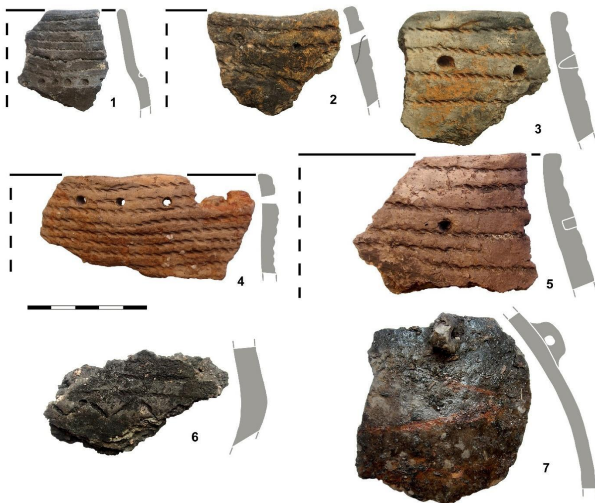
Fig. 6. GAC pottery from Daktariškė 5, western Lithuania. National Museum of Lithuania: 1 - VIII, 2 - X4b, 3 - III4a, 4 - III6b, 5 - V7a, 6 - without number, 7 - V6a1.
