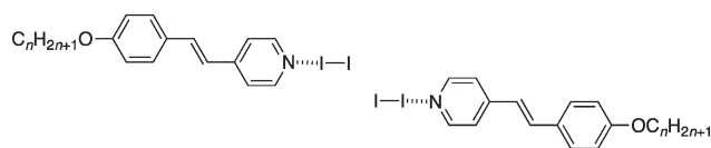
Fig. 1 Liquid-crystalline materials formed by iodine complexes of alkoxytilbazoles. The diagram shows the relative disposition of pairs of complexes as found in the solid state.
