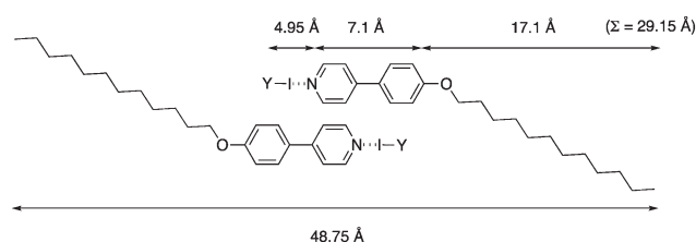
Fig. 16 Sketch to show maximum extent of likely overlap of the halogen-bonded liquid crystals, with distances based on the structures of 4-OPhPy \cdots I 2 Br and of [12-OPhPyH] + Br – .
