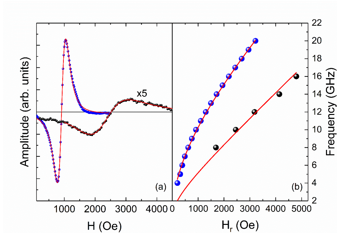
Figure 5: (a) FMR absorption measurement at 10 GHz for the as-grown (black data points) and annealed (blue) films. (b) Kittel curves (frequency vs resonant field) for the as-grown (black) and annealed films (blue).
