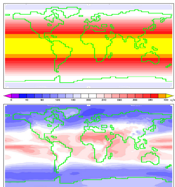
Figure 2 Annual insolation reaching the Earth's surface after passing through the atmosphere. Credits: This image was produced by William M. Connolley using HadCM3 data and is available at: https://commons.wikimedia.org/wiki/File:Insolation.png .
