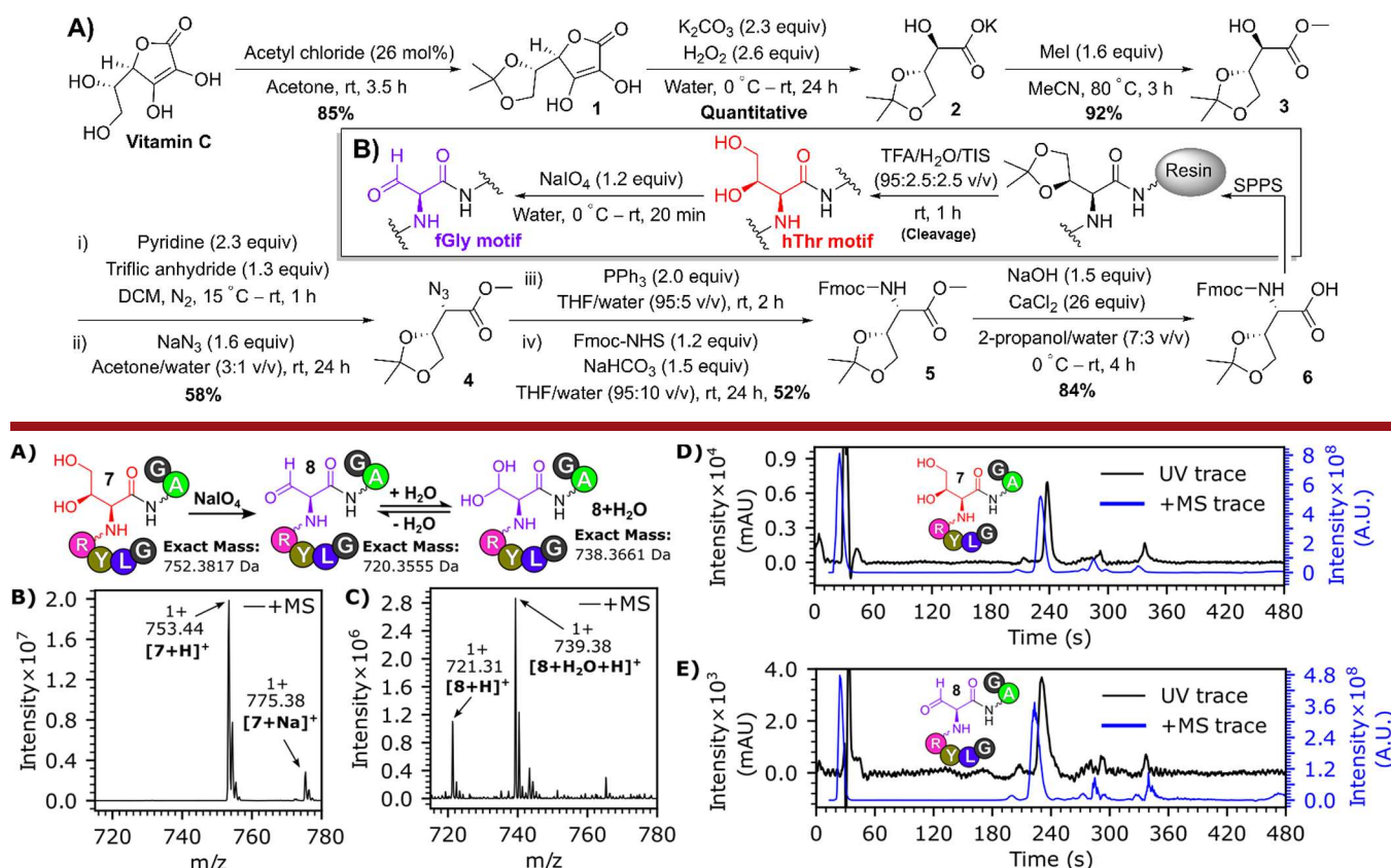
Figure 1. (A) Conversion of peptide 7 into peptide 8 using NaIO_4 . (B) MS analysis of 7. (C) MS analysis of 8. (D) LC-MS chromatogram of 7. (E) LC-MS chromatogram of 8. LC-MS chromatograms show the BPC+All MS trace and the UV chromatogram shows the absorbance for wavelengths 210–400 nm. LC-MS was conducted using LC gradient A (see Figure S1).
