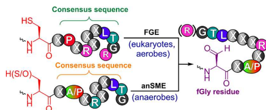
Scheme 1. Oxidation of Cysteine or Serine Residues by Either FGE or anSME Enzymes to Yield Formylglycine Residues 1b,3–5
