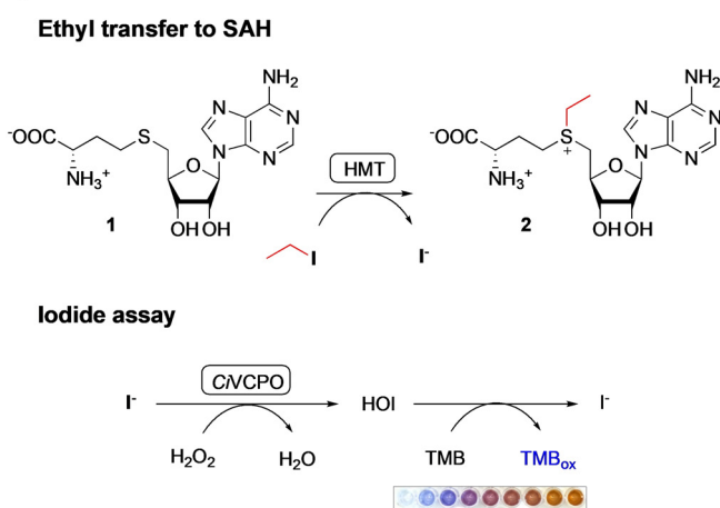
Figure 1. a) The crystal structure of AtHMT and the modelled alkyl iodides in the active site. The selected mutated sites, SAH, and the alkyl iodides, which include MeI, EtI, PrI, and BuI, are shown as sticks with elemental coloring. The carbons of SAH, MeI, EtI, PrI, and BuI are shown in white, grey, purple, yellow, and pink, respectively. b) Transfer of the ethyl group from ethyl iodide to SAH ( 1 ) and the production of SAE ( 2 ) and iodide. The iodide produced can be detected using hydrogen peroxide, a haloperoxidase, and TMB.
