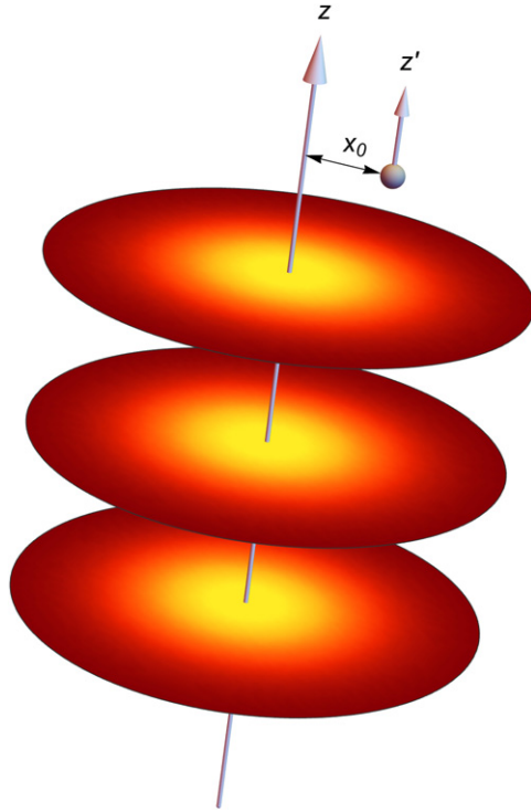
Figure 1. An atom displaced a distance x_0 from the z -axis of a Gaussian beam. This beam has flat phase fronts and therefore the orbital angular momentum about the beam's z -axis is zero. The orbital angular momentum about the atom's axis z' is also identically zero, as orbital angular momentum is intrinsic, and therefore we must ask from where the atom can obtain the two quanta of angular momenta required to drive the stated quadrupole transition.
