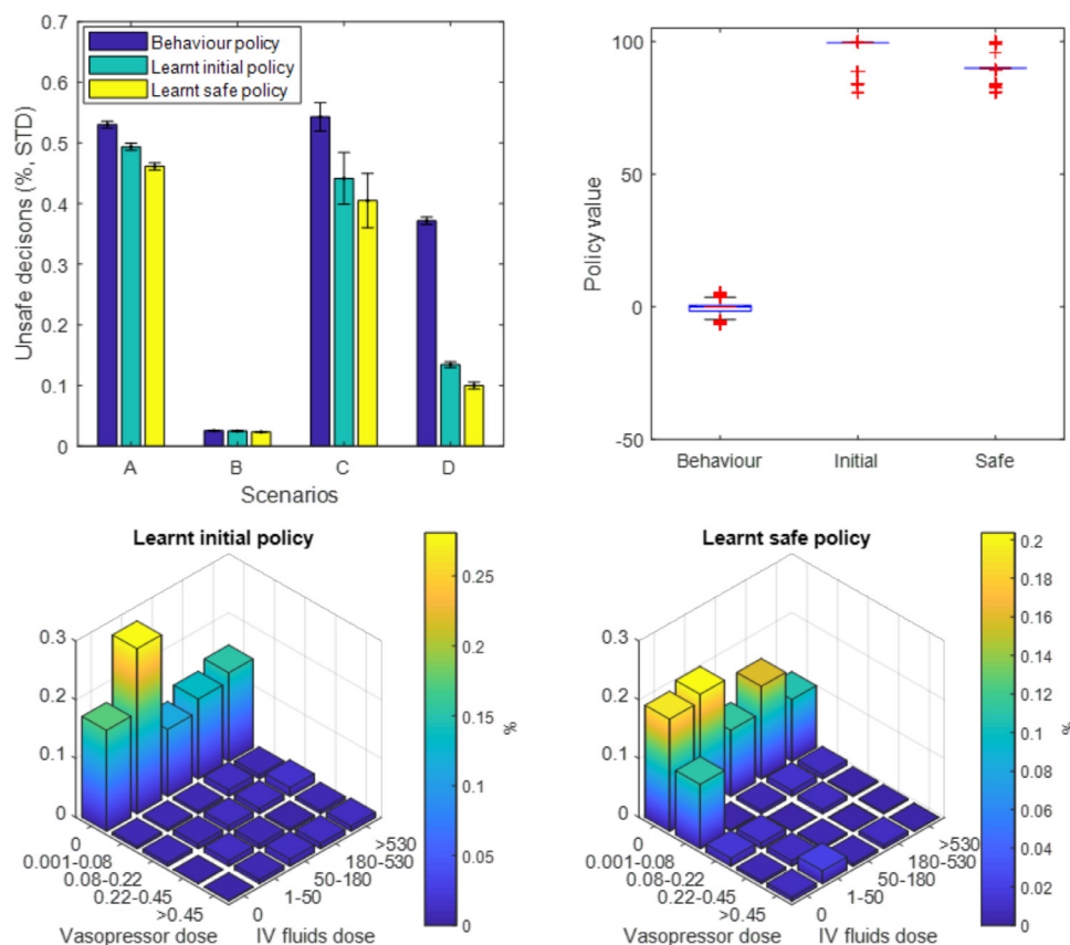
Figure 4 Results from the model retraining with added safety constraints. (A) Proportion of unsafe decisions in the four scenarios (see text) for three agents: human clinicians (behaviour policy), the original AI Clinician (learnt initial policy) and the modified AI Clinician (learnt safe policy). The original AI Clinician has a lower proportion of unsafe behaviour than human clinicians, while the modified 'safe' policy does better than the original AI Clinician. (B) Off-policy policy evaluation of the original and the modified AI Clinician policies. The value of the modified policy, with the added safety constraints, is slightly lower than the unrestricted policy (median, IQR): 90 (89.2–90) for the modified policy versus 99.5 (99.5–99.5) for the original policy, both being higher than the clinician's (0, –1.5 to 0.6). Bottom: distribution of 25 actions for initial (C) and improved (D) policies. The safe AI policy recommends more low-dose vasopressors, likely to try and correct instances of hypotension left untreated.
