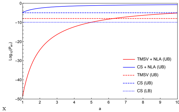
FIG. 5: Error probability exponents for QI using a maximally-entangled TMSV source with a sub-optimal NLA (red, solid) at the receiver, compared to a coherent state source with the same NLA (blue, solid). We consider a non-ideal NLA whose probability of success is half the maximum, P_{\text{succ}}^{\text{NLA}} = 1/(ag^2) , and results are plotted as function of the parameter a . Also included are associated upper bounds without the use of the NLA (dashed) showing how the NLA enhances this upper bound. The lower bound for coherent states (blue, dotted) shows the point beyond which a quantum enhancement (through the NLA, entanglement, or both) may be confirmed. As before, we have set N_B = 0.1 , \kappa = 0.2 and are considering low-energy applications with N_S = 0.01 . All probabilities are evaluated at M = 10^4 .
