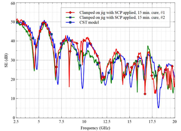
Fig. 12. Comparing the CST model for shield 2 with measured results.
