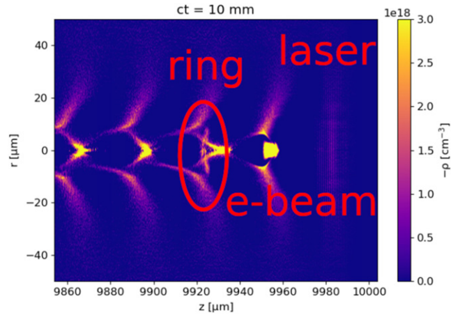
Figure 8. Electron density distribution obtained using FBPIC shows both the ring-shaped and the on-axis electron beams produced by a laser pulse with an initial a_0 = 1.35 focused inside the gas cell (at z = 3 mm). This snapshot is taken after 10 mm propagation.
