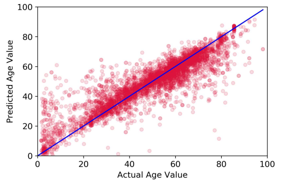
(b) XGBoost
