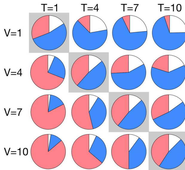
Figure 3. Pie charts for the cumulative number of released virions and TIPs 100 days post infection. Increasing the MOI of tiRNA (T) increases the cumulative number of released TIPs and reduces the total number of released particles (virion+TIP) compared with the control. Red and blue indicate the number of virions and TIPs, respectively, while white shows the difference between the total number of released virions in the control (tiRNA-free) case with the number of released particles (virion+TIP) in the presence of treatment. This figure is plotted by averaging over 250 simulations using parameter values from Table 1 with b_a = 1 and b_r = 1 . The initial condition for the MOIs of V = m , T = n is (+)\text{vRNA}^{\text{cyt}} = m , (+)\text{tiRNA}^{\text{cyt}} = n , and C_p = 180(m + n) .
