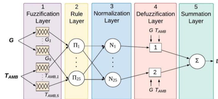
Figure 7. ANFIS architecture.
