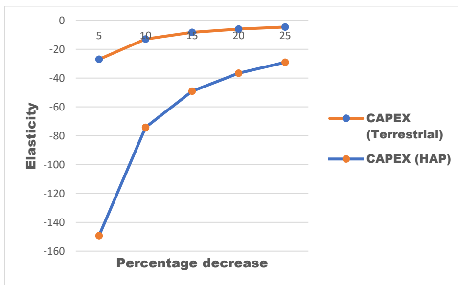
Figure 12: A graph of elasticity against percentage decrease in CAPEX for HAP and terrestrial systems
