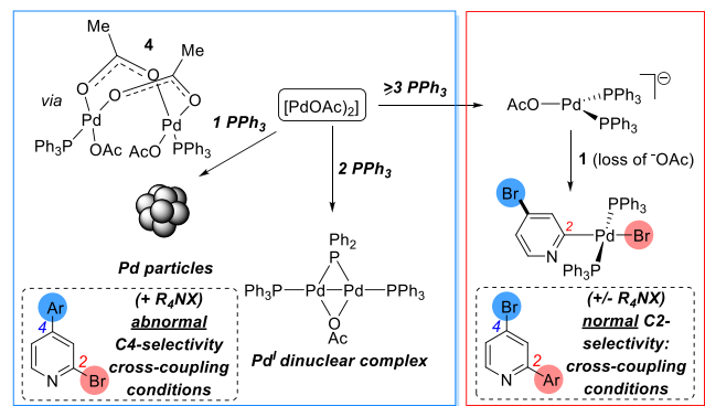
Scheme 8. Dichotomy in Site-Selectivity at 1: Different Pd Species Arising from Different Ratios of Pd(OAc) 2 / n PPh 3 Result in Different Cross-Coupling Selectivities under Cross-Coupling Conditions
