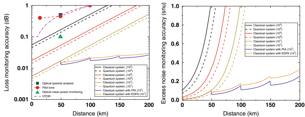
Fig. 2 Monitoring uncertainty at different distance. Monitoring uncertainty for channel loss (a) and quantum excess noise (b). For the classical system, the electronic noise is 0.4 shot noise, and the excess channel noise is 0.1 shot noise. For the quantum system, the electronic noise is 0.015 shot noise, and the excess channel noise is 0.01 shot noise. The PIA is a quantum-limited phase-insensitive amplifier. The inversion factor of the EDFA is set to 1.5. The detector efficiency is set to 0.4. The accuracy results for the classical monitoring system are as follows: \pm 0.1 dB for optical mean power monitoring (OMPM) 2 , \pm 0.5 dB for optical spectral analysis (OSA) 3 , 0.4 dB at 50km for a pilot tone 3 , and moderate sensitivity at a short distance (0.1 dB) but poor sensitivity at a long distance (0.05 dB/dB) 4,9 for OTDR. The noise is normalized to units of system shot noise (snu)
