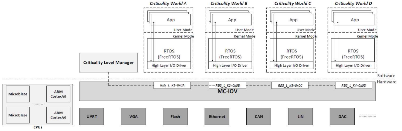
Fig. 1. MCS-IOV Architecture
