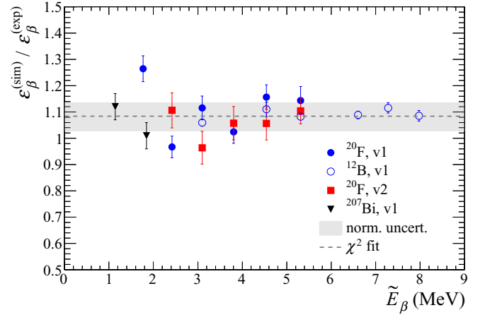
FIG. 5. Ratio of simulated and experimental transmission efficiencies, \epsilon_\beta^{(\text{sim})}/\epsilon_\beta^{(\text{exp})} , versus the central energy selected by the magnetic transporter, \tilde{E}_\beta . The data are labeled by the isotope ( ^{12}\text{B} , ^{20}\text{F} , ^{207}\text{Bi} ) and the detector (v1, v2) used for the measurement. The gray band indicates the systematic uncertainty on the normalization of the ^{20}\text{F} data. The dashed line was obtained from a \chi^2 fit to the data in which the normalization of the ^{12}\text{B} data was allowed to vary freely (see text for details).
