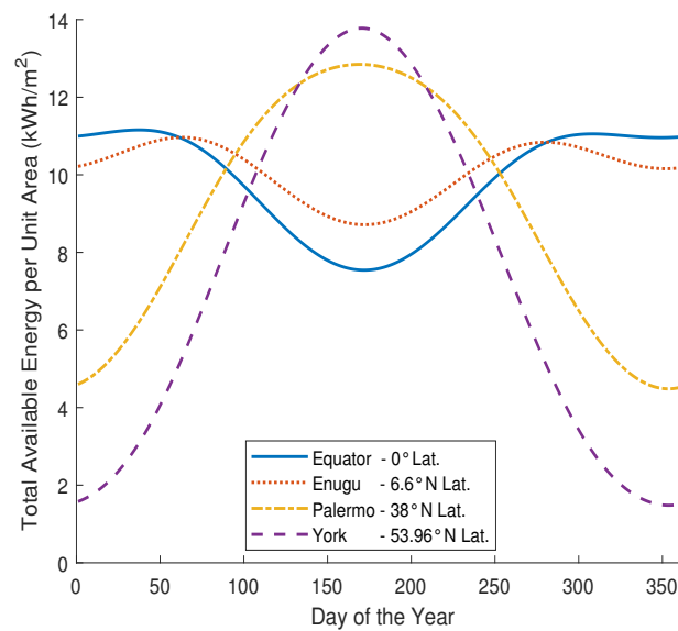
Figure 8. Total solar irradiance per m^2 at various locations for a given day of the year highlighting the longer days in northern hemisphere.
