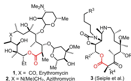
Figure 1. Macrolide antibiotics 1–3.
