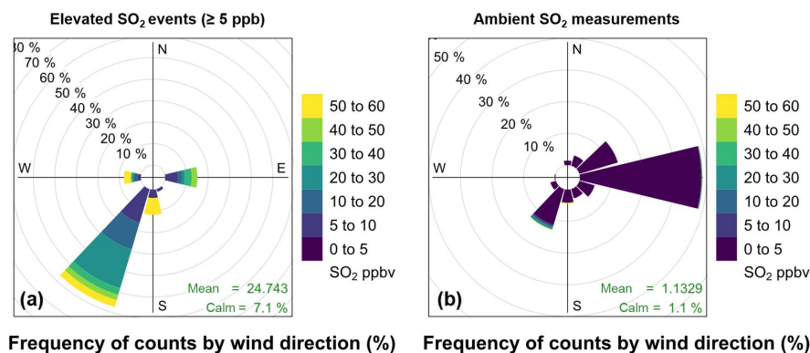
Figure 5. Pollution rose plots to show the relationship between wind direction and SO 2 concentration at the Bachok measurement site. Panel (a) represents recorded SO 2 concentrations \geq 5 ppb and panel (b) represents all SO 2 data recorded during the measurement period. Plot constructed using the openair package in RStudio (Carslaw and Ropkins, 2012; Carslaw, 2015).
