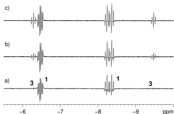
Figure 3. Hydride region of a series of ^1\text{H} NMR spectra of a solution of 1 in \text{C}_6\text{D}_6 in the presence of 10 fold excess \text{AsPh}_3 under p\text{-H}_2 at room temperature showing hyperpolarized signals for 1 and 3 after: a) 1 laser shot, b) 2 laser shots and c) 4 laser shots.
