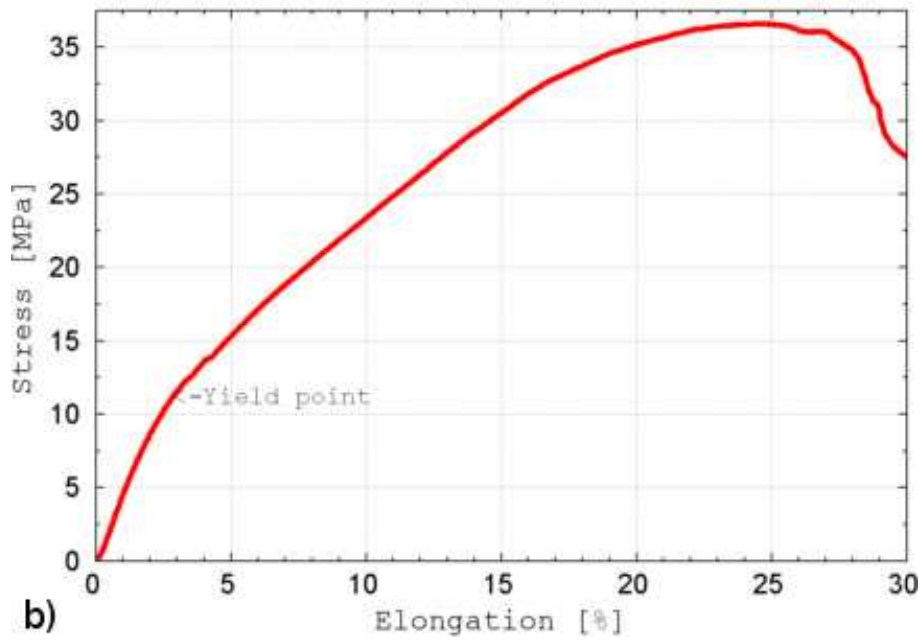
Figure 4: Tensile testing of the recycled HDPE: a) experimental setup (0.40 mm strand shown); and b) the resulting tensile stress-strain curve.
