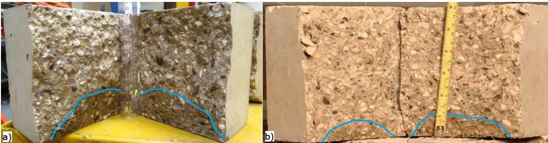
Figure 8: Comparison of the water penetration depths on the 150 mm cubes made of (a) plain concrete and (b) FRC mix C5 (with 0.40% of \varnothing 0.40 mm HDPE fibres).
