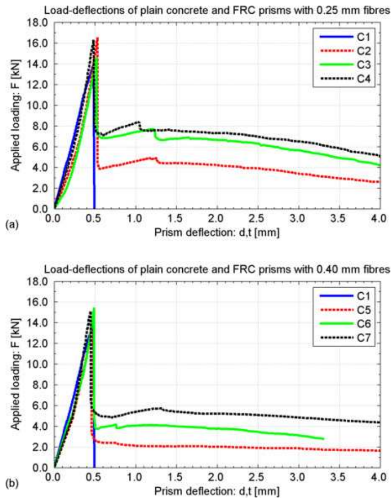
Figure 6: Flexural ductility of plain concrete (C1) and HDPE FRC with: a) \text{Ø}0.25 \text{ mm} fibres (C2-C4); and b) \text{Ø}0.40 \text{ mm} fibres (C5-C7).
