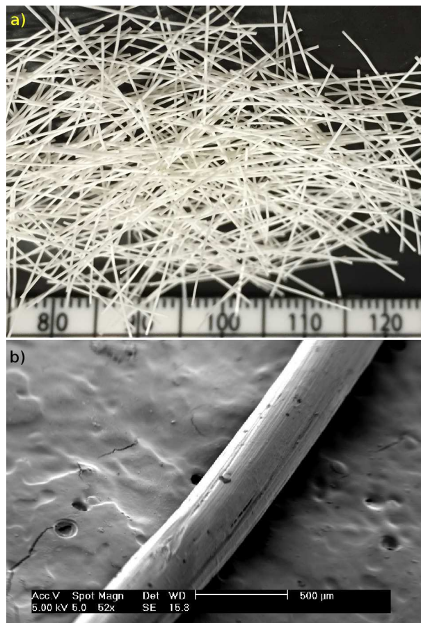
Figure 2: \varnothing 0.25 \text{ mm} HDPE fibres: a) actual look ( mm scale); and b) SEM 52 \times magnified image of a single fibre.
