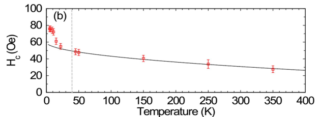
FIG. 5. (Color online) The temperature dependence of the coercivity measured along [01]. The line is a fit to Sharrock's equation, the departure from which is clear below 40 K (which has been indicated with the dotted line).
