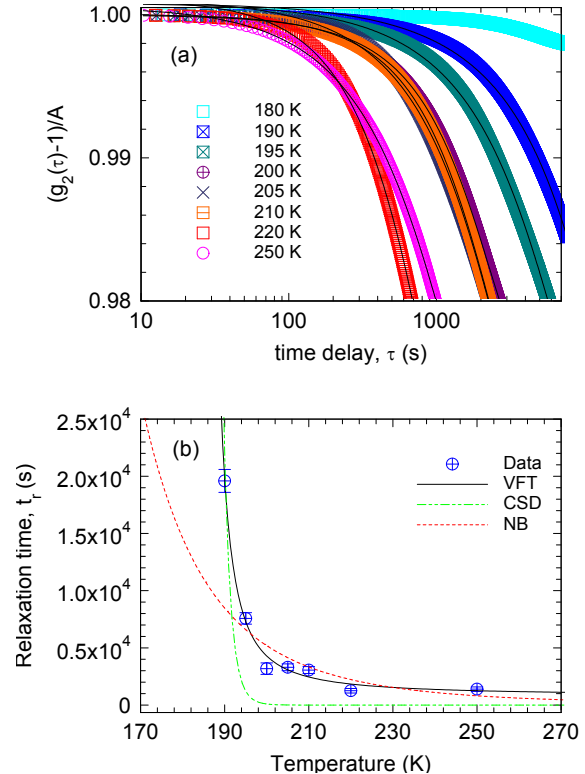
FIG. 3. (Color online) XPCS results. (a) Normalized g_2(\tau) functions at various temperatures. The lines are fits to Eq. 2. (b) Relaxation times t_r as a function of temperature, fitted by a Vogel-Fulcher-Tammann (VFT) law. Also plotted is the superparamagnetic Néel-Brown (NB) law and critical slowing down (CSD) law near a phase transition, which fit poorly. Data points for T = 180 K (where t_r \gg 10^5 s) and T = 295 K (where t_r \lesssim 5 s) are not plotted since the experimental constraints mean that determining values within these bounds was not possible.
