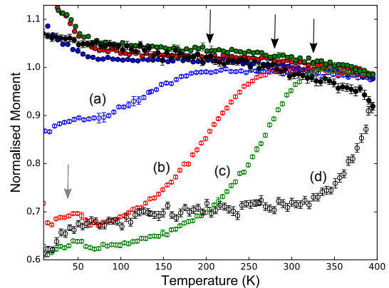
FIG. 4. (Color online) ZFC (open circles) and FC (filled circles) magnetization measurements under different applied magnetic probe fields of (a) 50 mT, (b) 35 mT, (c) 25 mT and (d) 5 mT. The average blocking temperature, T_B , is also defined by the maximum in the ZFC curve and is indicated by the black arrows ( T_B > 400 K at 5 mT). The grey arrow indicates the \sim 40 K feature in the ZFC data. The field was applied along [01] direction of the ASI lattice.
