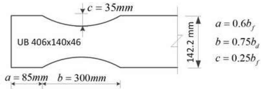
(b) Geometrical size of the RBS zone according to EC8 [8]
