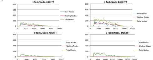
Figure 15: The effect of multi-tasking on improvement of the performance of an FFT task model.
