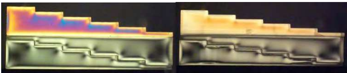
Fig. 4 Dark-field fringe information of the side profile of the staircase blocks for the build-up layers, 16µm (left) and 32µm (right) In this case, the blocks are being viewed in the X-Y plane which yields residual strain in block 1, as the staircase build layers are stacked in this plane, causing the shrinkage of the block to be most prominent
