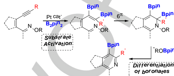
Scheme 1. The diboration-6 \pi -electrocyclization strategy.
