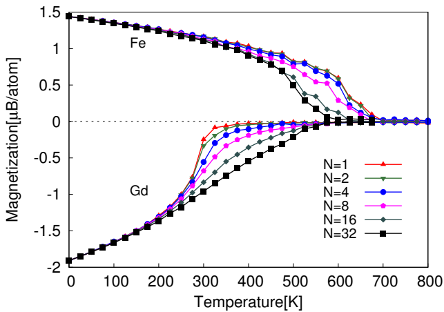
Figure 2. (Color online) Numerically calculated magnetization curves of each sublattice for the Gd/Fe multilayers as a function of temperature. Results are shown for a range of the number of repeats of the layers.
