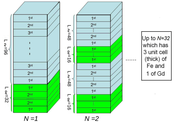
Figure 1. (Color online) Schematic of the Gd/Fe multilayered structures.
