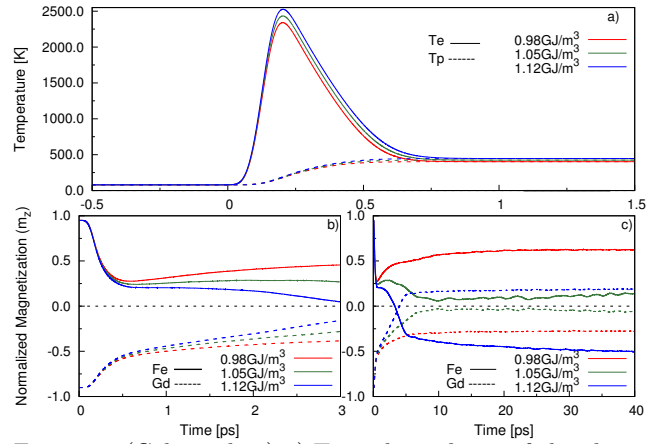
Figure 3. (Color online) a). Time dependence of the electron and phonon temperature from the two-temperature model. b). and c). Ultrafast magnetization dynamics curves for the Fe (solid lines) and Gd sublattices (dashed lines) for a range of pump fluences for 32 repeats ( N = 32 ) at short delay time in b) and at long delay time in c). Note the three different timescales for the electron/phonon (a) and magnetization (b) / (c) dynamics.
