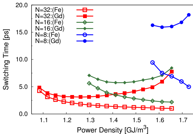
Figure 5. (Color online) Switching times of both Fe sublattice and Gd sublattice as a function of the laser energy for samples N = 8 , N = 16 and N = 32 .
