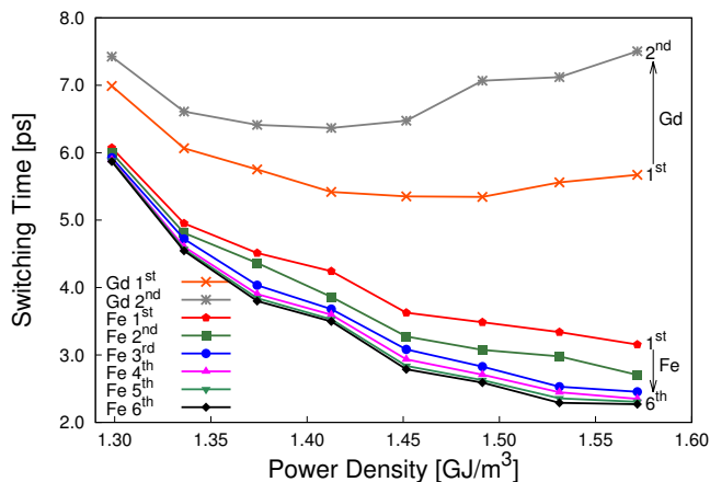
Figure 6. (Color online) Layer resolved reversal times for each Fe and Gd plane in the N = 16 structure. The direction of the arrows represent the direction away from the interface to the central plane. The numbers represent the plane index where 1 st is the interface plane up to the central plane (2 nd for Gd and 6 th for Fe).
