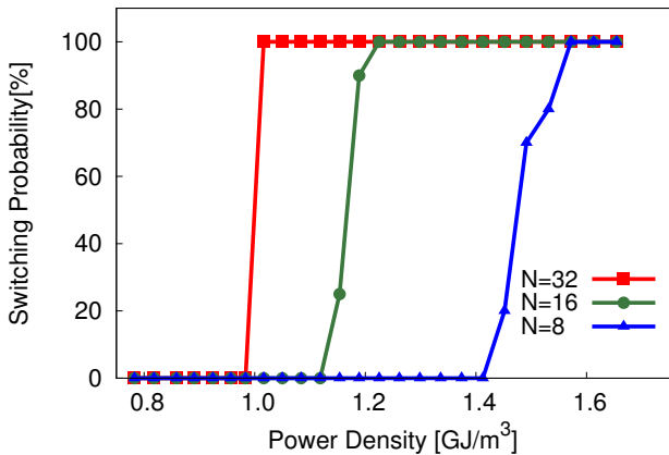
Figure 4. (Color online) Numerically calculated the switching probability as a function of the laser energy for samples N = 8 , N = 16 and N = 32 .
