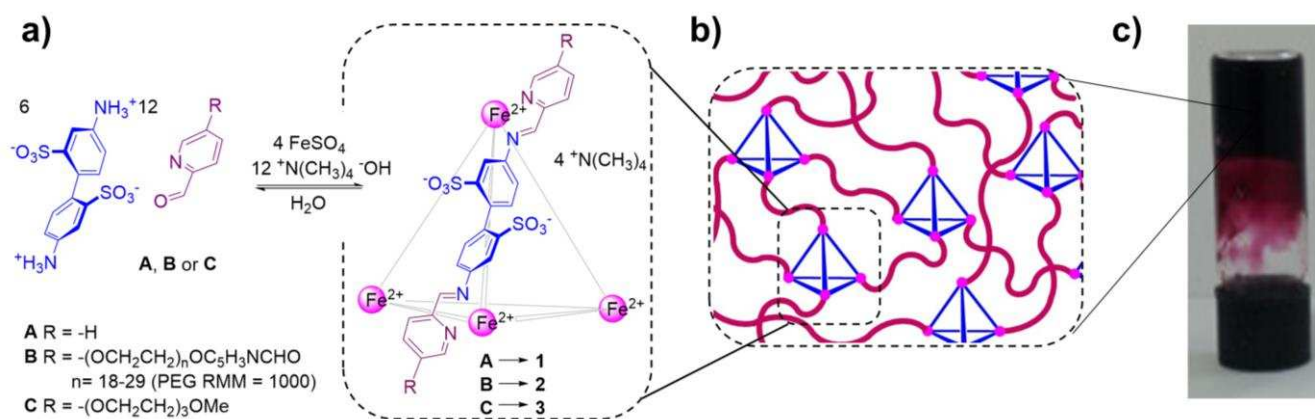
Figure 1. Metal-organic cage cross-linked hydrogel formation: (a) synthesis of cages 1-3 using aldehydes A-C , and (b) a schematic view of the structure of the cage-cross-linked gel. (c) A photograph showing an inverted vial containing a 15 wt% hydrogel formed by cage 2.
