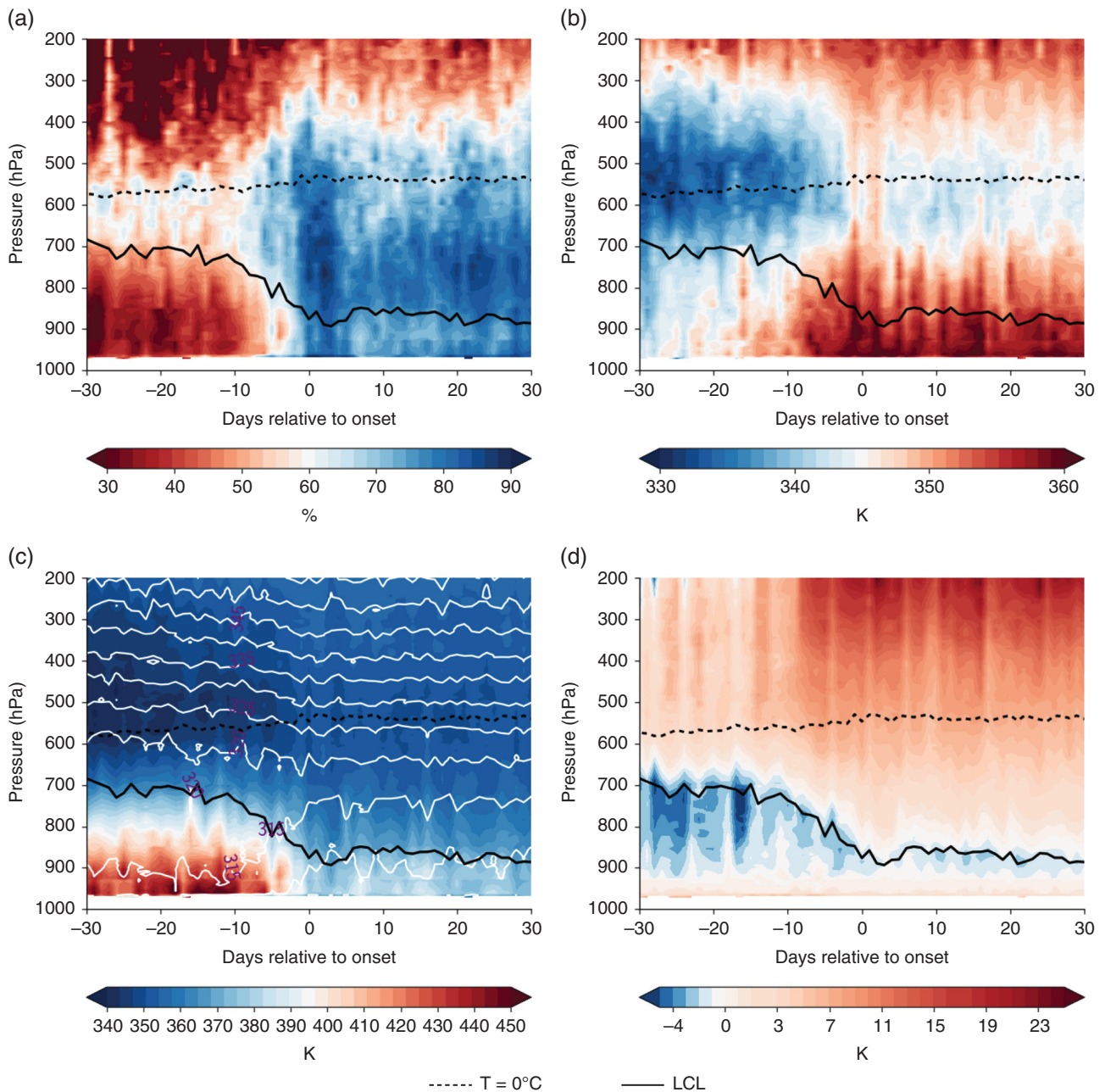
Figure 8. Time–pressure sections for Nagpur showing (a) RH (%), (b) \theta_e (K), (c) \theta_{es} (K) with virtual potential temperature \theta_v , overplotted (contours, K) and (d) buoyancy of lifted boundary-layer parcels (K). All panels show LCL (solid line) and level of T = 0^\circ\text{C} (dotted line). The profiles are computed for days relative to the onset date at this station on each year (Day 0 in the time axis) for the period 1991–2015: over this period, the mean arrival of the northern limit at this station is 16 June.
