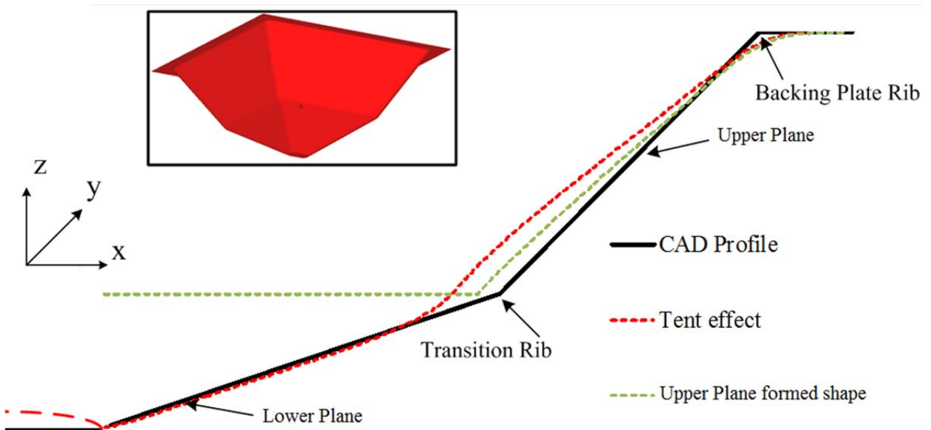
Fig.6. Conventional tent effect phenomenon illustrated for the forming of a two slope pyramid; the green dotted line shows the shape formed at the end of forming the top planar face and the red dotted line shows the shape formed at the end of forming the lower plane; the tent effect occurs as a result of pulling of the top plane by the bottom plane when the bottom plane is being formed
