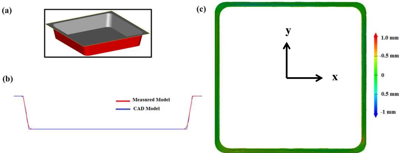
Fig.3. Truncated pyramid of wall angle 80° and depth 35 mm formed with accuracy in the range [-0.572 mm, 0.787 mm] shown in isometric view in (a), section at x=0 compared in (b) and accuracy color plot shown in (c)
