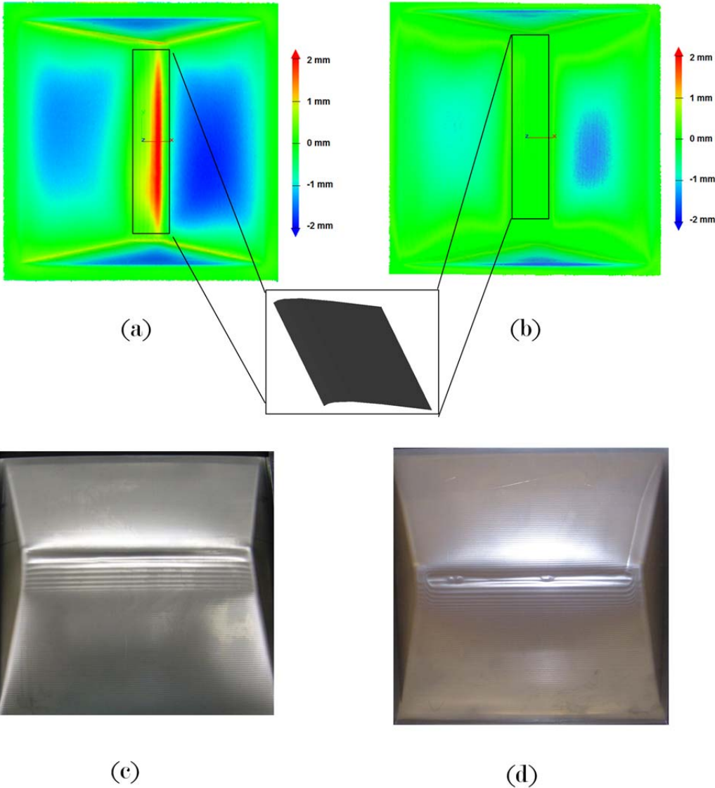
Fig.19. Airfoil manufacture and accuracy results showing: (a)-(b) color plots of accuracy for (a) AISI 304 part made with uncompensated toolpath (d) AISI 304 part made with a morphed surface; rectangular inset in each color plot shows the section of the airfoil (c)-(d) shows the actual manufactured parts made with (c) AISI 304 uncompensated (d) AISI 304 made with the integrated morphing strategy
