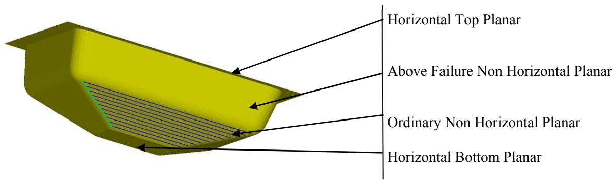
Fig.13. Example of a feature specific partial tool path made on the ordinary non horizontal planar feature
