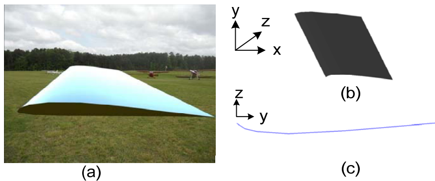
Fig.17. Airfoil design (a) picture of original model of airfoil [19] (b) STL model of the airfoil (c) cross-section of the airfoil taken at X=0 in the co-ordinate system shown for (b)
