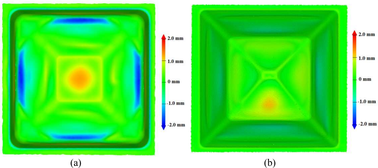
Fig.16. Accuracy plots of truncated pyramids made with morphed tool paths in combination with intelligent sequencing of tool paths for (a) pyramid with wall angles 80^\circ and 25^\circ (b) pyramid with wall angles 60^\circ and 30^\circ
