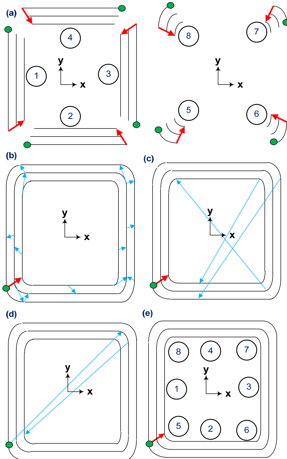
Fig.14. Sequencing of tool paths showing (a) feature tool paths for planar features (1-4) and ribs (5-8) (b) tool axis sequencing errors (c) xy-plane sequencing errors (d) step down sequencing errors (e) correctly sequenced tool paths ( errors are shown with blue lines; the direction of arrows indicates the directionality of the tool path in the z-axis; the green circles indicate the start points of the tool paths )
