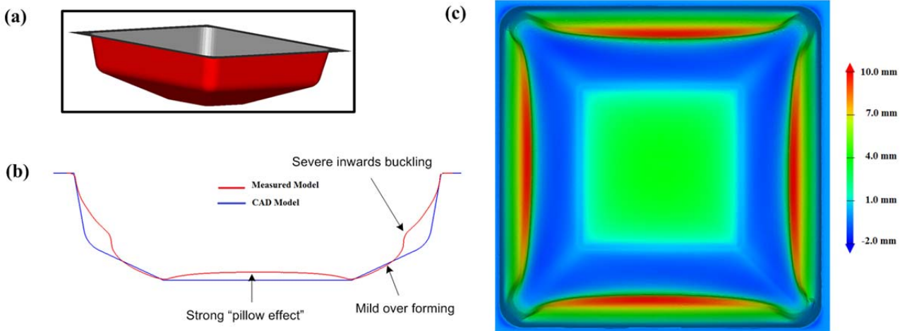
Fig.5. Two slope truncated pyramid of top plane wall angle 80^\circ and depth 35 mm formed in combination with bottom plane with wall angle 25^\circ and depth 17.5 mm with accuracy in the range [-1.243, 10.04 \text{ mm}] shown in isometric view in (a), section at x=0 compared in (b) and accuracy color plot shown in (c)
