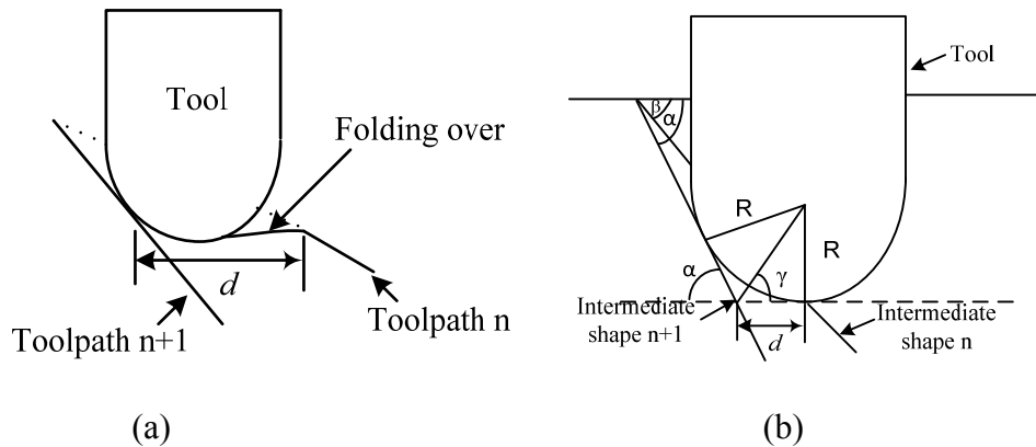
Fig.7.(a) Folding over effect at too large offset between successive tool path passes, (b) Maximum offset between successive tool paths in multi-step processing of parts
