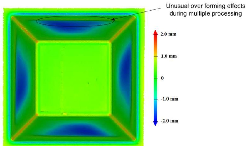
Fig.4. Effects of multiple processing on a pyramid of wall angle 70° made with AA 1050 of 1.5 mm
