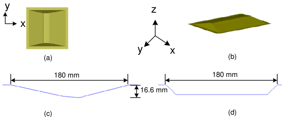
Fig.18. Extended airfoil model for manufacture showing (a) top view in xy plane (b) isometric side view (c) sectional view at X=0 (d) sectional view at Y=0
