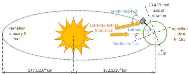
Fig. 2. Illustration of the geophysical parameters controlling Irradiance .
