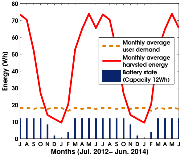
Fig. 4. Average daily harvested energy and user demand aggregated over a month and the corresponding average battery state. \lambda_U (user density) = 6\lambda_M (metro-cell density), \alpha = 4 , \lambda_{LP} = 0.48 \times 10^{-3} (Nottingham) and \sigma^2 = -90 dB/Hz.
