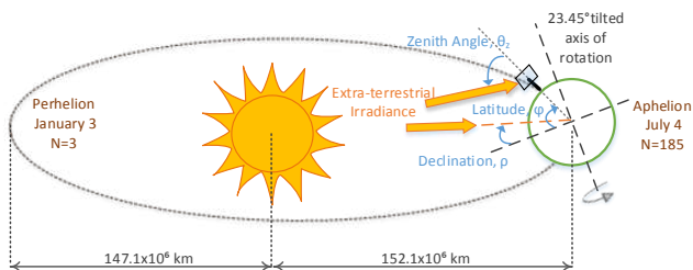
Fig. 2. Illustration of the geophysical parameters controlling Irradiance .
