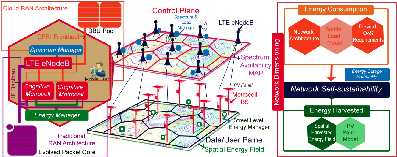
Fig. 1. 5G Cognitive Metro-Cellular Network Architecture.
