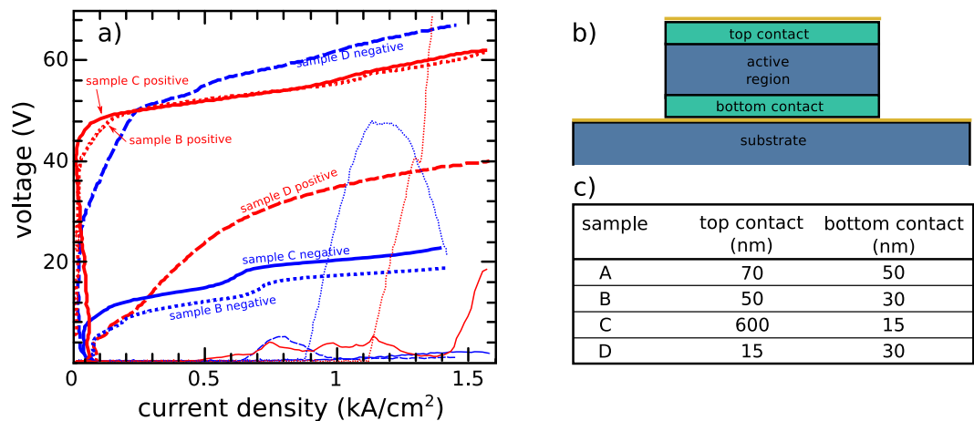
Figure 3. Samples performance. (a) IV characteristics of samples B (dotted line), C (solid line) and D (dashed line) in positive (red) and negative (blue) polarity. (b) Sketch of the sample cross-section. Positive polarity is defined as positive voltage applied on the top contact. (c) Summary of the contact layer thicknesses for all investigated samples.
