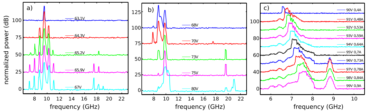
Figure 4. Microwave emission spectra. Microwave emission spectra, measured at different bias voltages and at a heat sink temperature of 70 K, for (a) sample B, and (b) a nominally identical non-lasing device belonging to the same epitaxial growth (dimensions 760 \times 140 \mu\text{m} ). The samples were mounted on the cold finger of a helium continuous-flow cryostat and driven in pulsed mode with 200 ns pulses and 10 kHz repetition rate. (c) Microwave emission measured at room temperature at various bias conditions for a 360 \times 140 \mu\text{m} device, similar to sample B, biased with 400 ns pulses at a 1 kHz repetition rate.
