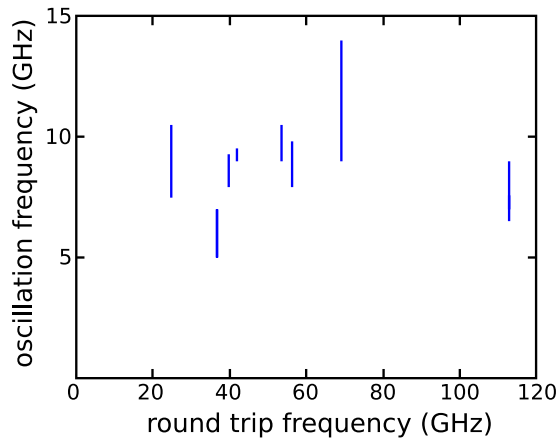
Figure 5. Microwave emission vs round trip. Microwave emission frequencies collected from a set of different samples. The vertical lines mark the microwave emission bandwidth, and their location on the x-axis corresponds to the cavity round-trip frequency of the corresponding QCL device.
