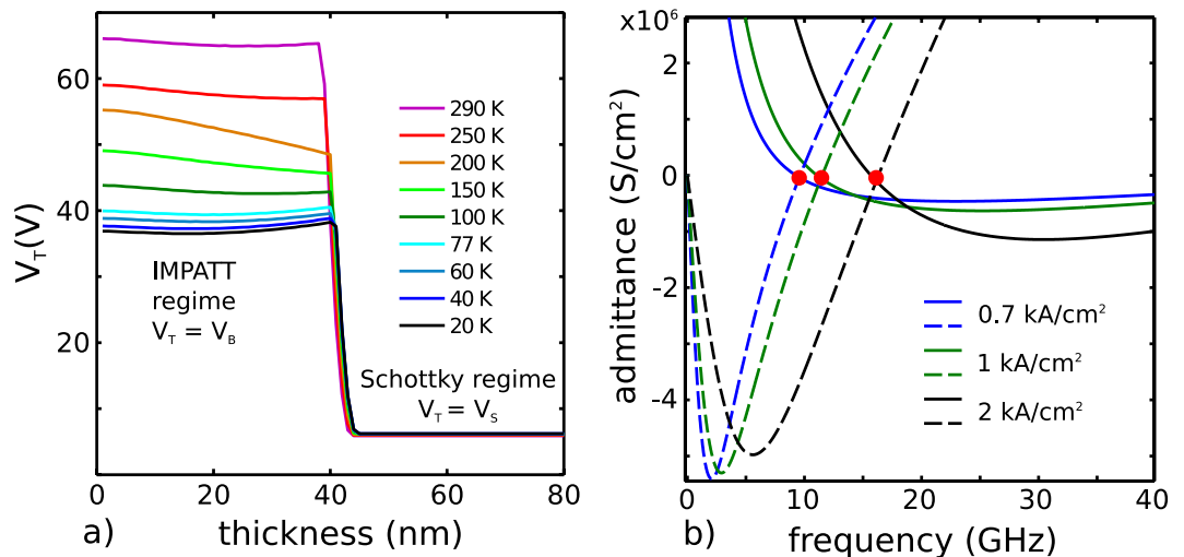
Figure 8. Modelling. (a) Injection threshold voltage of sample B calculated as a function of the contact layer thickness and heat sink temperature. (b) Real (solid lines) and imaginary (dashed lines) parts of the admittance of the injection diode of sample B calculated for different bias current densities, as a function of frequency. The red dots mark the resonance frequency, defined as the beginning of the negative resistance region.
