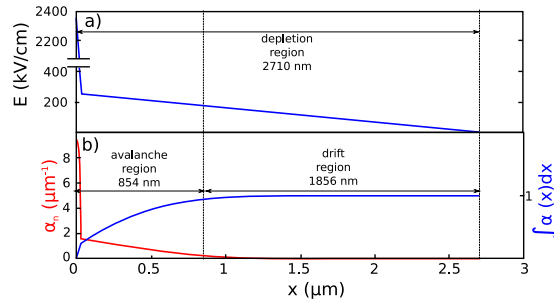
Figure 7. Modelling. (a) Static electric field as a function of the distance x from the metallic contact in the depletion region of sample B. (b) Impact ionization generation rate (red) and ionization integral (blue). The calculations were performed at a temperature of 20 K and at an applied bias voltage of 37 V, corresponding to the avalanche breakdown voltage.
