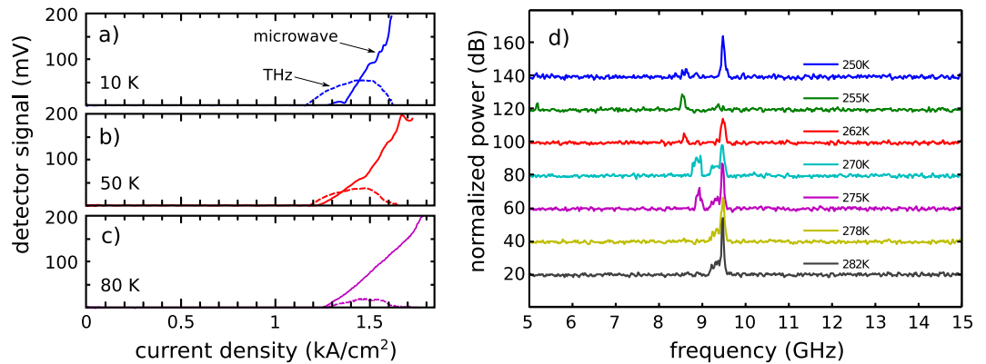
Figure 2. Terahertz and microwave emission. (a–c) Microwave (solid line) and THz (dashed line) components of the light-current characteristics of sample B, measured at heat sink temperatures of (a) 10 K, (b) 50 K, and (c) 80 K. Being the responsivity of the pyroelectric detector unknown in the microwave regime, the vertical axis shows the raw voltage signal read by the pyroelectric sensor, which is proportional to the emitted radiation intensity. (d) Microwave emission spectrum of a sample B collected at heat sink temperatures in the range 250–285 K. The sample was biased in pulsed mode (200 ns pulse width and 10 kHz repetition rate), and the displayed microwave power is normalized to the noise floor of the spectrum analyzer.
