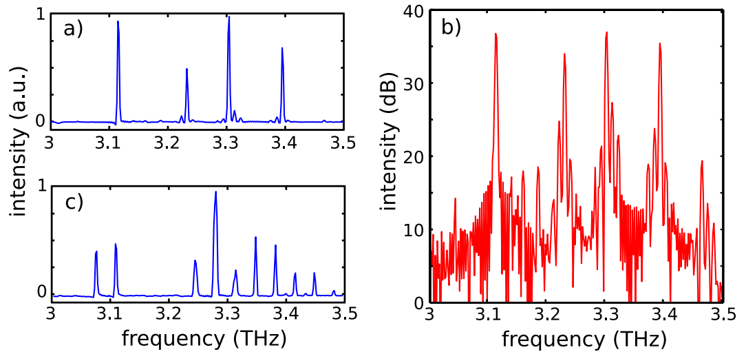
Figure 6. Frequency and amplitude modulation. THz emission spectra of sample B on a (a) linear and (b) logarithmic scale, measured at a heat sink temperature of 70 K and whilst driving the QCL with a 65 V bias. The spectra were measured while the QCL was operating in pulsed mode (200 ns pulses, 20 kHz repetition rate) using a Fourier transform infrared spectrometer equipped with a helium-cooled Si bolometer, with a spectral resolution of 0.125 \text{ cm}^{-1} , corresponding to 3.7 GHz in rapid-scan mode.
