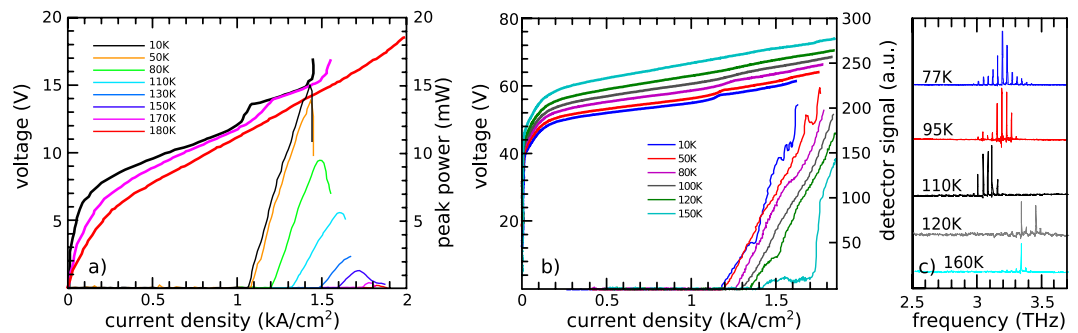
Figure 1. Electrical and optical characterization. (a,b) Current-voltage (thick lines, left y axis) and light-current (thin lines, right y axis) characteristics of the (a) reference sample A (dimensions 1200 \times 180 \mu\text{m} ), and (b) sample B having a 30 nm thick injection contact (dimensions 1720 \times 140 \mu\text{m} ). Being the responsivity of the pyroelectric detector unknown in the microwave regime, the vertical scale in (b) shows the raw voltage signal read by the pyroelectric sensor. (c) Emission spectra of a sample from the same batch of sample B (dimensions 1100 \times 140 \mu\text{m} ) at different heat sink temperatures. All measurements were performed in pulsed mode by driving the QCL with a 200 ns pulses and at a 10 kHz repetition rate.
