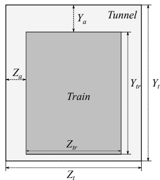
Figure 7: Diagram of blockage ratio variation parameters (cross sectional view).
