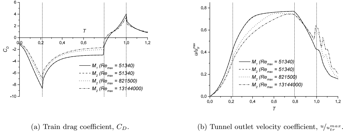
Figure 4: Train drag and tunnel outlet velocities for the models M_1 and M_2 .
