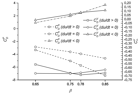
Figure 10: Pressure ( C_D^P ) and viscous ( C_D^V ) drag coefficients.
