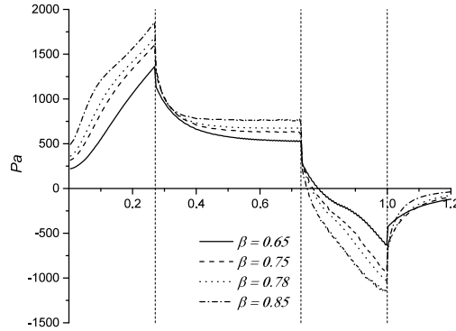
Figure 9: Pressure difference between train front and back.
