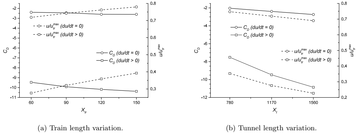
Figure 12: C_D and u/u_{tr}^{max} for train length variation for two phases of motion.
