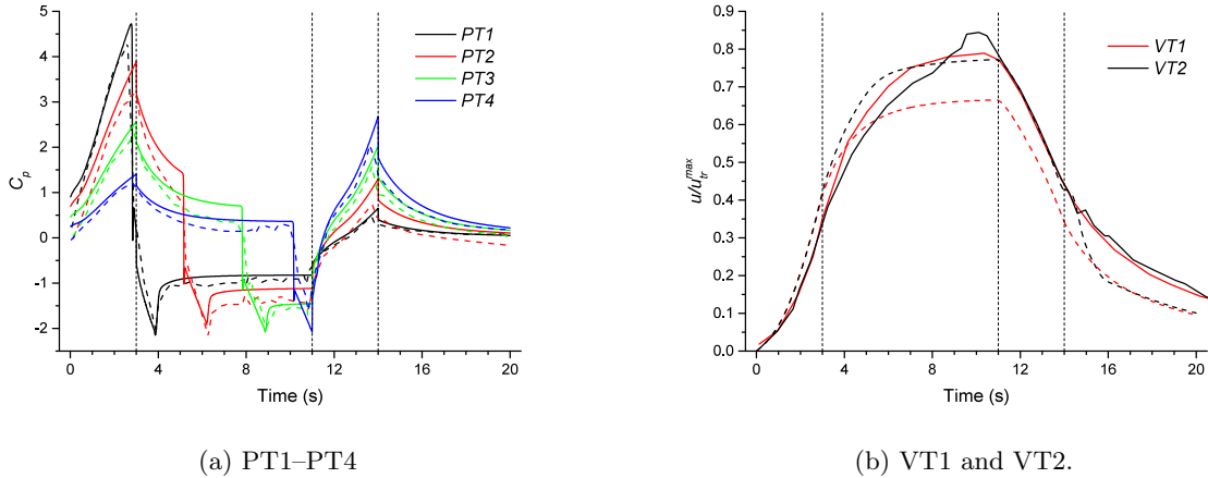
Figure 3: Pressure and velocity coefficients at the positions shown in Figure 1 (— Numerical result, - - Experimental result).
