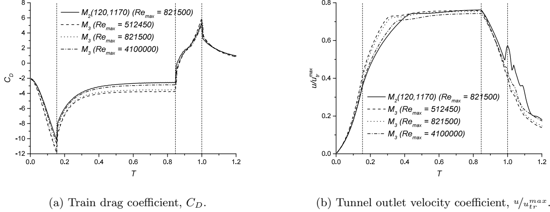
Figure 5: Train drag and tunnel outlet velocities for models M_2 and M_3
