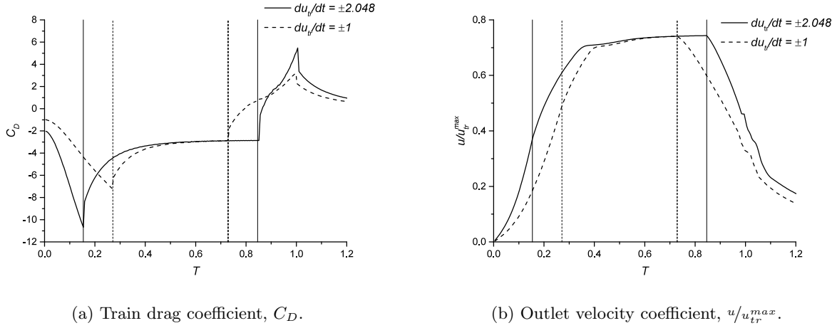
Figure 6: Results for du_{tr}/dt variations for model M_3 with Re_{max} = 4.100 \times 10^7 .
