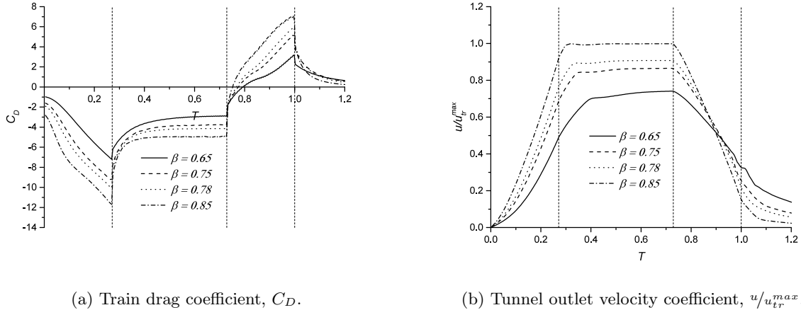
Figure 8: Train drag and tunnel outlet velocities for various blockage ratios.
