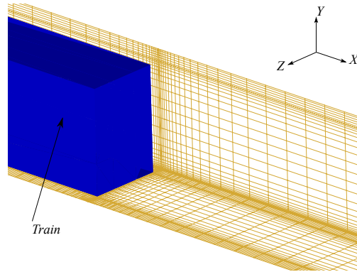
Figure 2: Hexahedral grid around the train front.
