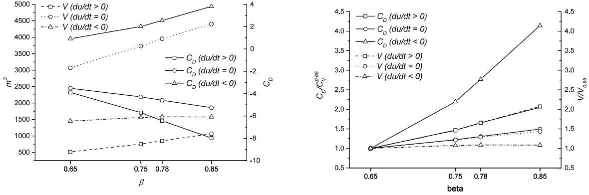
(a) Tunnel outlet air flow volume ( V ) and average train drag coefficients ( C_D ). (b) Normalised coefficients, ( V/V^{0.65} ) and ( C_D/C_D^{0.65} ).
