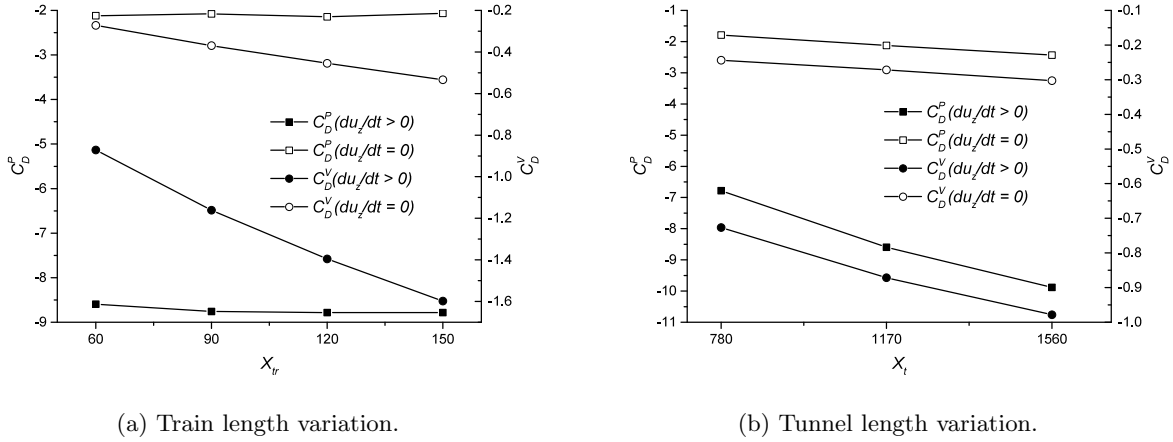
Figure 13: C_D^P and C_D^V for train and tunnel length variation.
