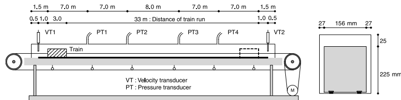
Figure 1: A schematic diagram of the Kim and Kim [8] train and tunnel scale model experimental set-up.
