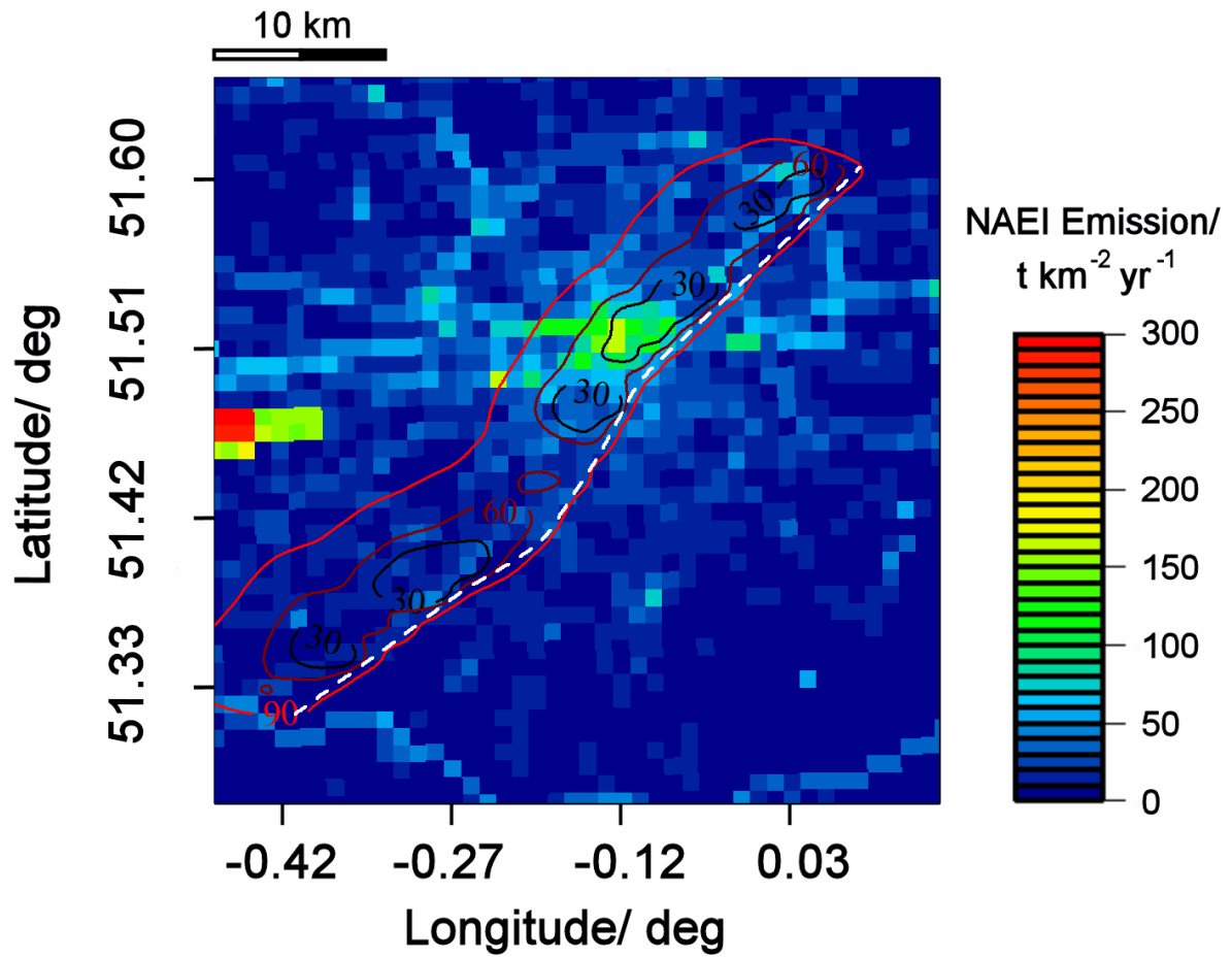
Figure 3. The contributing footprint area to a typical flight track, dependant on the prevailing wind direction and altitude of flight. The footprint is overlaid onto the NAEI at 1 \text{ km}^2 grid resolution, coloured to annual \text{NO}_x tonnage emission estimates.
