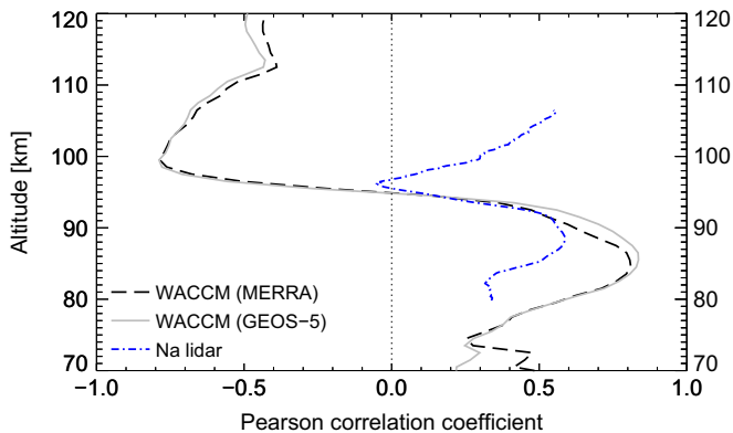
Fig. 6. Pearson correlation coefficient between diurnally averaged Na number density and temperature versus altitude in km. Grey solid line: WACCM-Na nudged to GEOS-5. Black dashed line: WACCM-Na nudged to MERRA. Blue dash-dotted line: Na lidar. The vertical dotted line marks a correlation coefficient of 0.0. Na lidar data have been averaged over six altitude bins (i.e. 900 m). (For interpretation of the references to color in this figure caption, the reader is referred to the web version of this article.)
