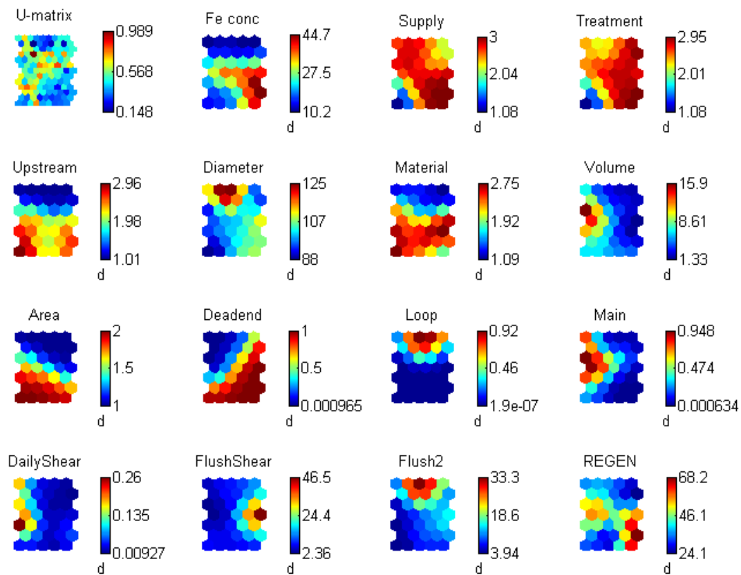
Figure 6: SOM for regeneration fieldwork results with UK site determinants
