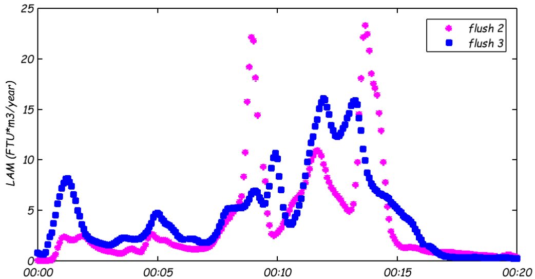
Figure 4: LAM per year for first return flush in March 2010 (17 months after initial flush) and second return flush in October 2010 (24 months after initial flush), flushing action 2 on mainly a 200 mm, 1000 m AC pipe, with flushing of 42 l/s (1.42 m/s) and 50 l/s (1.71 m/s).
