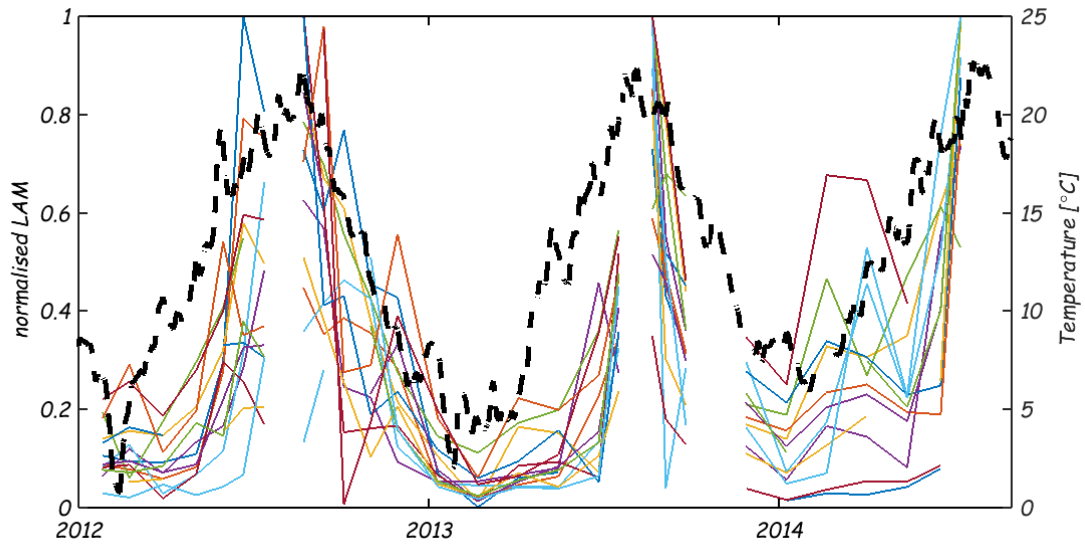
Figure 11: Dotted black line = calculated soil temperature at -1 m (validated with drinking water temperature samples). The other lines are the accumulation rates (per day) over time for all the flushing action locations, normalized to a maximum of 1.
