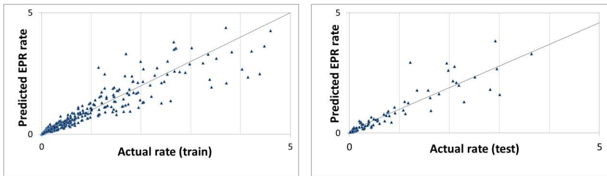
Figure 12: Scatter plots of the observed data and the EPR model-predicted regeneration rate (train and test for F-fold 5)
