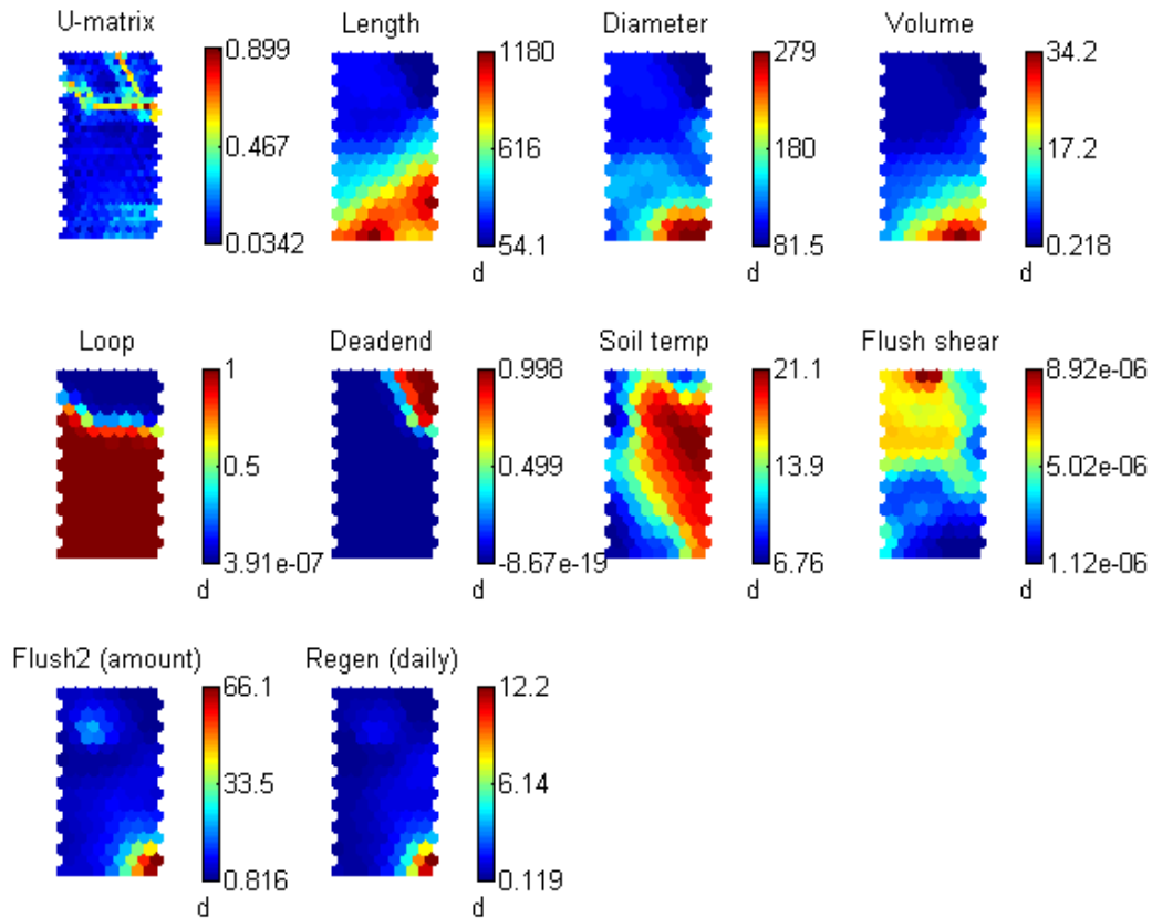
Figure 10: SOM for multiple flushing operations in Case Study 3
