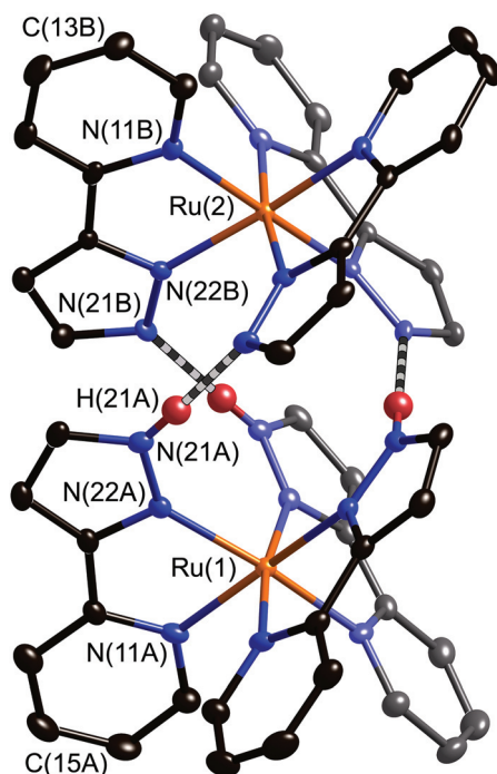
Fig. 6 Structure of the hydrogen-bonded dinuclear complex cation of fac -[Ru(L H ) 3 Ru(L - ) 3 ](PF 6 ) 3 ·3C 7 H 8 (thermal ellipsoids at 40% probability level). Some of the ligands are shown in paler colours for clarity; the hydrogen-bonds between the two complex units are indicated by the striped lines.
