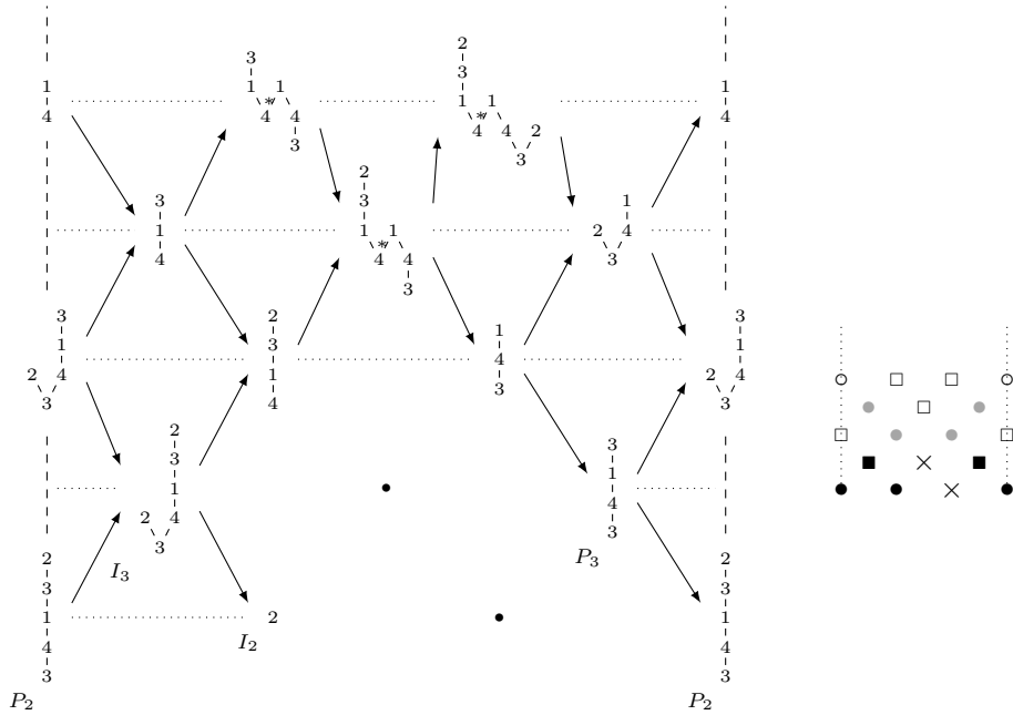
FIGURE 9. The left hand diagram shows part of the AR-quiver of \Lambda -mod. The right hand diagram shows the same objects. The symbol for a module is circular if it is Schurian, filled-in with gray if it is rigid but not \tau -rigid, and filled-in with black if it is \tau -rigid. The symbol \times represents a gap in the AR-quiver (corresponding to an indecomposable direct summand of \tau T )
