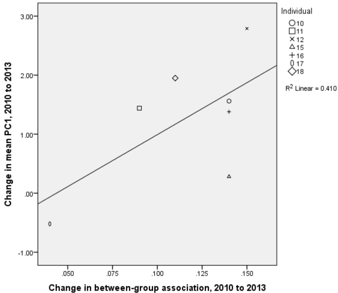
Figure S1. Scatterplot showing for each BB individual (N = 7) the relationship between the difference in mean PC1 between 2010 and 2013 (measure of acoustic change) and the change in between-group association for the same period. Between-group association was calculated from the dyadic composite association measures used in our Social Network Analysis [1], which comprised of rates of being in the same party and being nearest neighbours. In each year, for each BB individual we calculated a mean association value from all his/her dyadic association scores with each ED individual.
