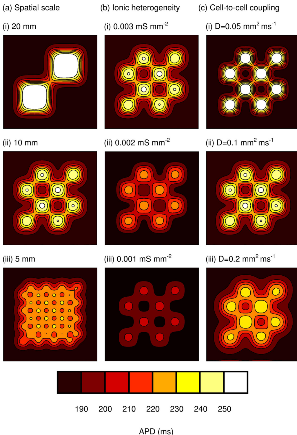
Figure 3 Spatial distribution of APD during from pacing at 500 ms intervals in each variant of the 60 × 60 mm virtual tissue. (a) Effect of changing spatial scale, with \Delta gK_{max} fixed at 0.003 mS mm -2 , and diffusion coefficient fixed at 0.1 mm 2 ms -1 . (b) Effect of changing \Delta gK_{max} , with spatial scale fixed at 10 mm, and diffusion coefficient fixed at 0.1 mm 2 ms -1 . (c) Effect of changing strength of cell-to-cell coupling by changing the diffusion coefficient, with spatial scale fixed at 10 mm, and \Delta gK_{max} fixed at 0.003 mS mm -2 .
