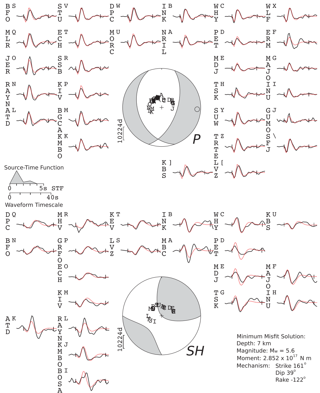
Figure 5. Telesismic waveform modeling solution for the earthquake on 3 July 1996. The method used is described in the text. Data are shown in black, synthetics for the minimum misfit solution shown in red. Spheres show lower hemisphere projections of the radiation patterns. Upper sphere and waveforms are for P waves, lower sphere and waveforms are SH waves.
