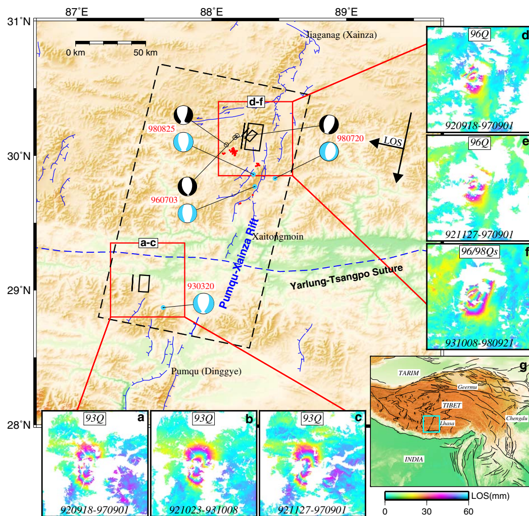
Figure 1. Topographic and tectonic map of the Pumqu-Xainza Rift, southern Tibet, and the observed coseismic radar interferograms. Tick marks on the rifts indicate hanging wall slip direction with faults from Kali [2010]. The dashed box delimits the extents of our radar data. The short and long arrows indicate radar looking and flight directions respectively. The colored circles and the “beach-balls” show the locations and the focal mechanisms of the four events from the GCMT (cyan) and NEIC (black) models respectively. The black boxes show the surface projections of InSAR-derived east-dipping fault models, with solid lines representing the fault trace. Red dots denote epicenters of the manually located earthquakes, which occurred in 2004–2005, from Monigle et al. [2012]. Portions of the coseismic interferograms in the red boxes are shown in Figures 1a–1c and 1d–1f respectively. Each fringe represents 60 mm of displacement in the satellite line of sight in these rewrapped interferograms. (g) Tectonic map of the Tibetan Plateau with faults from Taylor and Yin [2009]. Cyan box indicates the area of the main figure.
