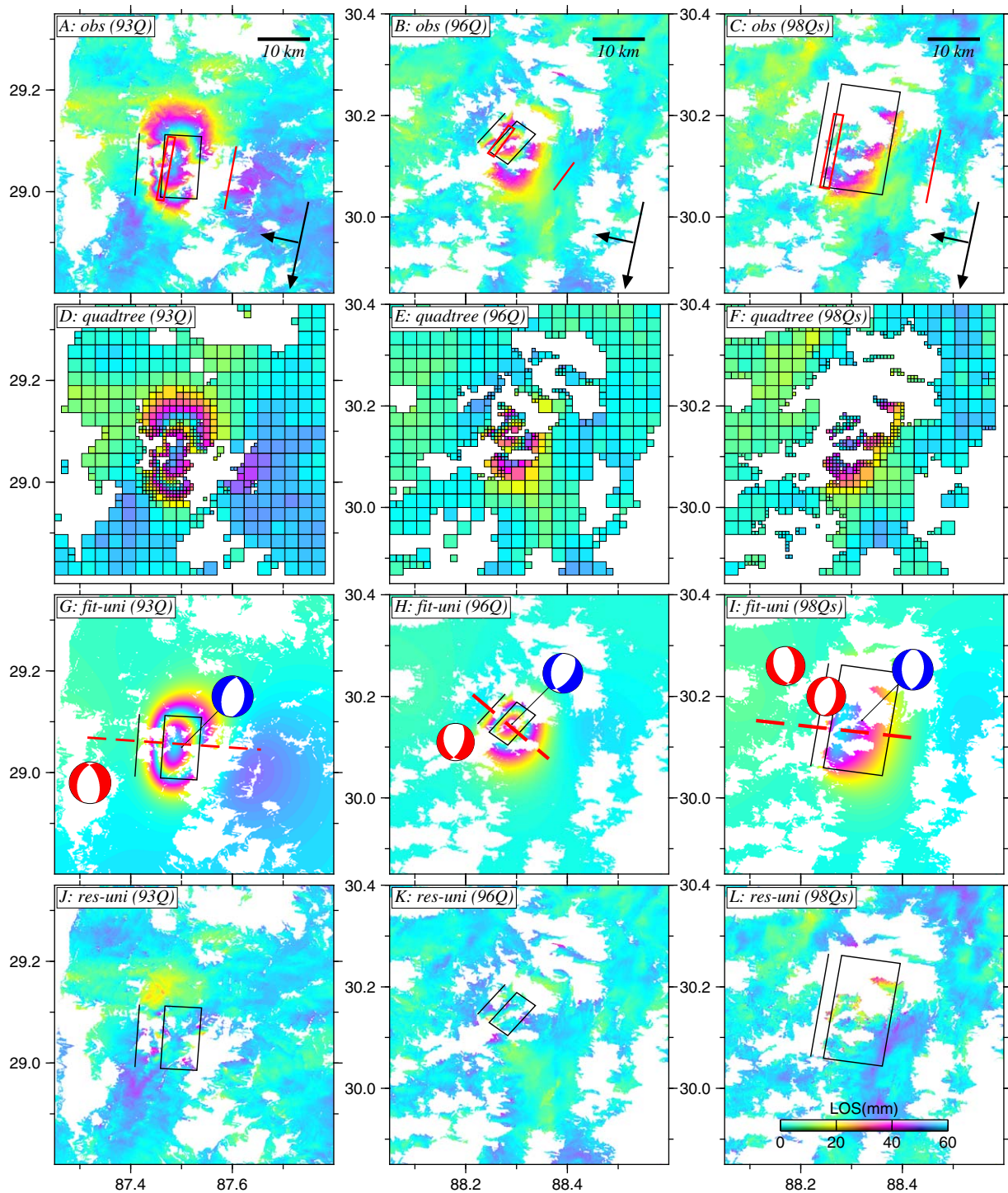
Figure 3. Stacked coseismic displacements and uniform slip modeling. (a) Coseismic interferogram for the 1993 event stacked using data in Figures 1a–1c. (b) Coseismic interferogram for the 1996 event stacked using data in Figures 1d and 1e. (c) Coseismic interferogram for the 1998 events using the difference between Figures 1f and 3b. The black and red boxes show the surface projections of the east and west-dipping fault models respectively, with solid lines representing the fault trace. The short and long arrows indicate radar looking and flight directions respectively. (d–f) Down-sampled observations using quadtree algorithm. (g–i) Synthetic interferograms from the east-dipping uniform slip models. The “beach-balls” denote focal mechanisms from BW (red) and ICMT (blue) solutions. (j–l) Residuals from the east-dipping uniform slip models.
